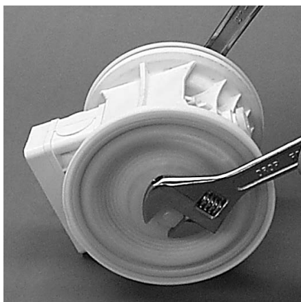
Step 11. Figure 11 Using two (2) 1" sockets, remove diaphragm assembly from center section assembly.
