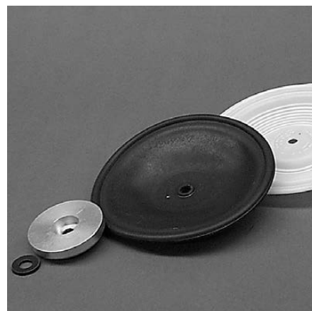
Step 13. Figure 13 Inspect diaphragms, outer and inner pistons and disc spring (not shown) for signs of wear. Replace with genuine Wilden parts, if necessary.
